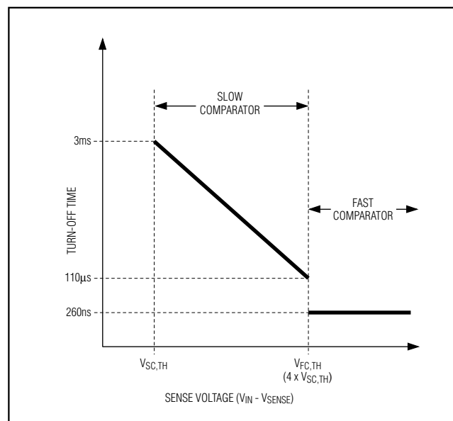
Figure 3. VariableSpeed/BiLevel Response
