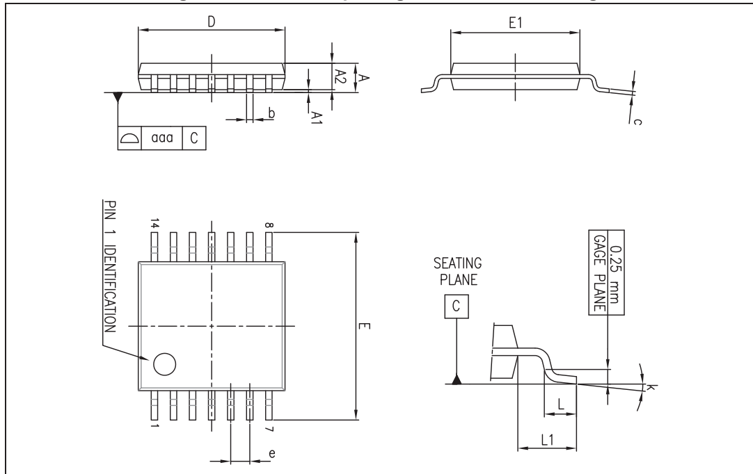
Figure 61. TSSOP14 package mechanical drawing
