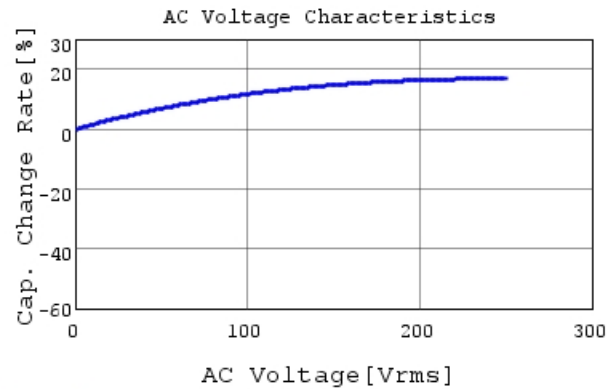
GA342DR7GF102KW02 C-AC Voltage capchange, Dc
